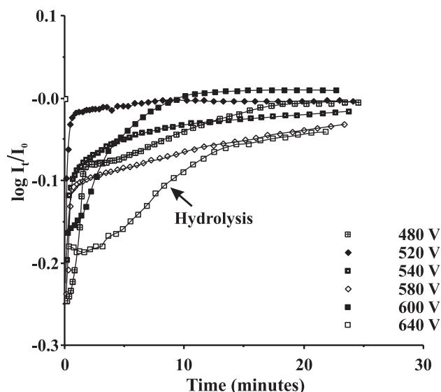
Fig. 6. Electrolysis caused by application of 50 \mu s pulses of various pulse heights in the range of 480–640 V in an isotonic saline solution.
