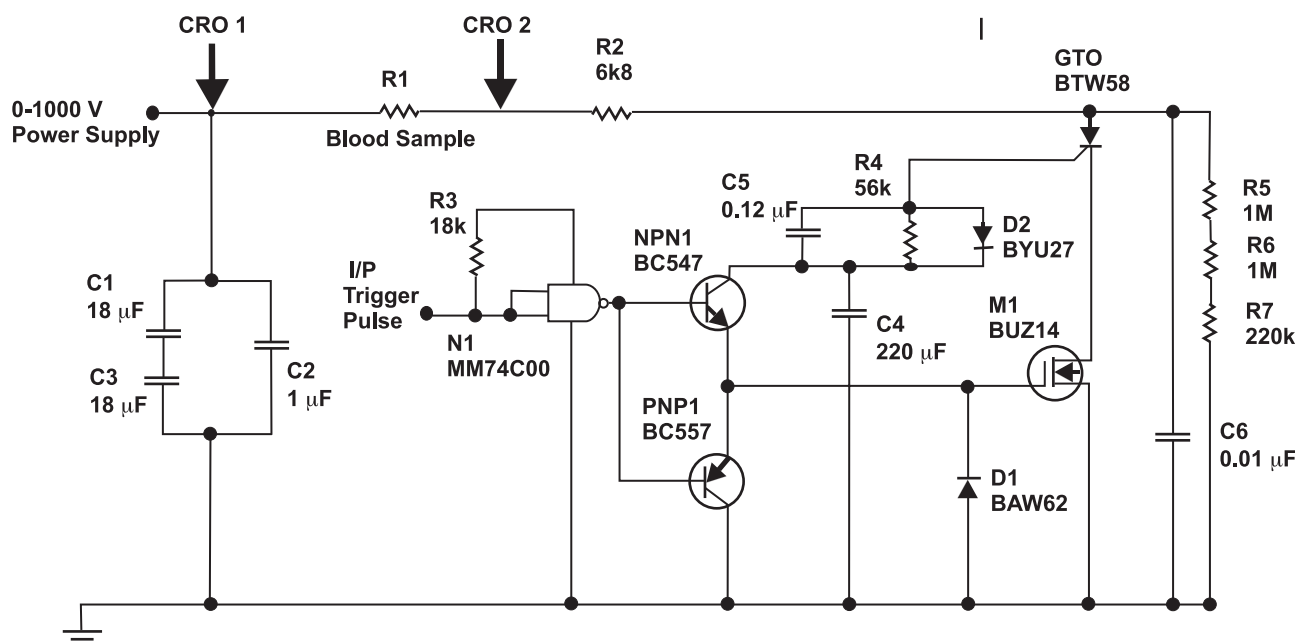
Fig. 13. The high voltage switching circuit. The input trigger pulse activates the MOSFET and GTO on and off, discharges the capacitors and applies an electric field across the erythrocyte suspension. The capacitors are not substantially discharged during the time that the switch is “on” so that the pulse height is essentially constant in time. The circuit is capable of providing pulses in the range between 5 \mu s to 5 ms in pulse length and up to 1 kV in height. By setting the desired voltage and pulse length, the circuit can deliver pulses with current flows of 25 A during the time the input trigger pulse is applied.
