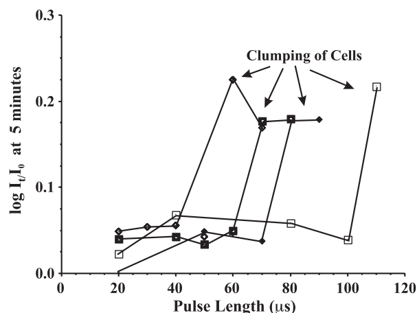
Fig. 11. The critical pulse length progressively decreased as the sample voltage was increased (data taken from a 5-min post-pulse haemolytic curve).
