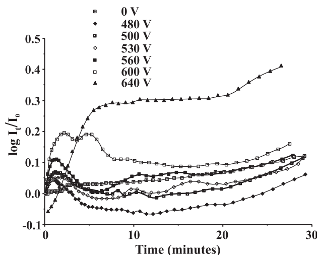
Fig. 7. The haemolytic curves obtained during a 30-min period using a 5 \mu s pulse and pulse heights of 0, 480, 500, 530, 560, 600 and 640 V.
