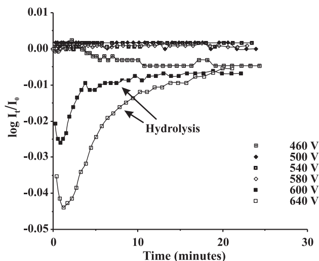
Fig. 5. Electrolysis caused by the application of 5 \mu s pulses with various pulse heights in the range of 460–640 V applied across the electrodes in an isotonic saline solution.
