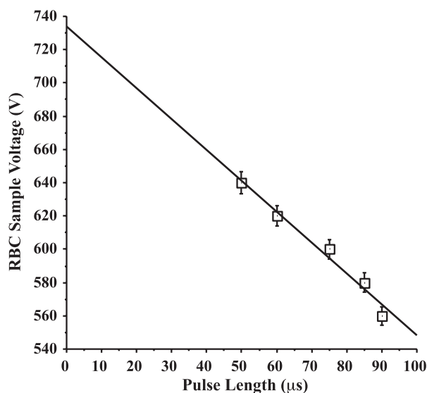
Fig. 12. A plot of the critical pulse length against pulse height applied to the RBC sample for a particular donor.
