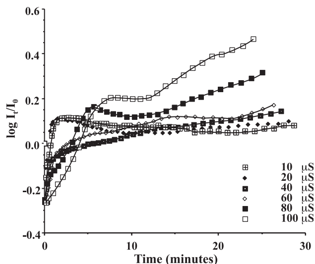
Fig. 9. The haemolytic curves obtained with a pulse of 600 V and pulse lengths of 10, 20, 40, 60, 80 and 100 \mu s.
