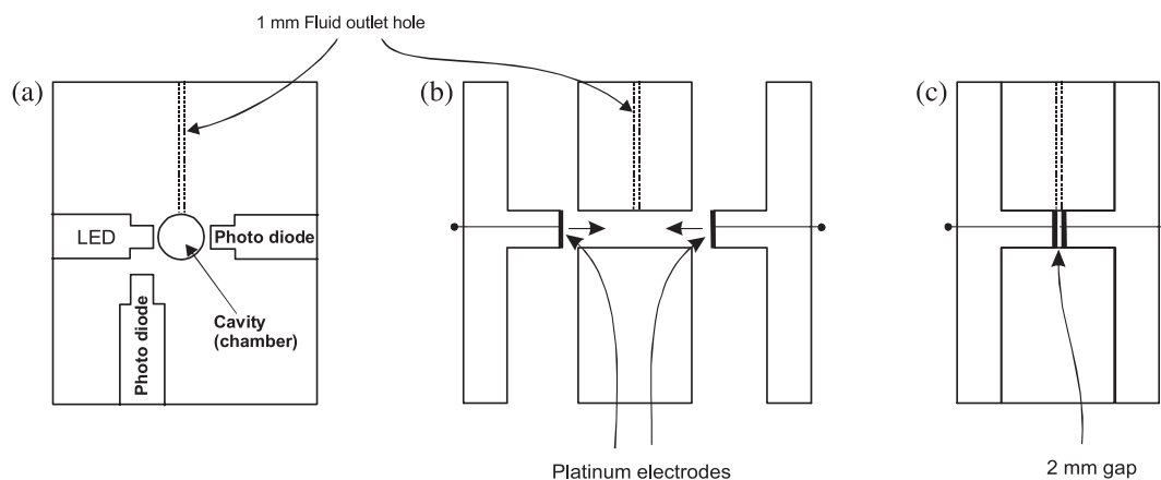
Fig. 1. A schematic diagram of the sample holder showing (a) a lateral view of the central plexiglass block designed to hold the photodiode–light emitting diode system, the sample (in the cavity) and the outlet fluid hole used for expulsion of excess liquid from the cavity; (b) an end elevation with each of the sections separated and; (c) an end elevation with each of the plexiglass sections fitted together.
