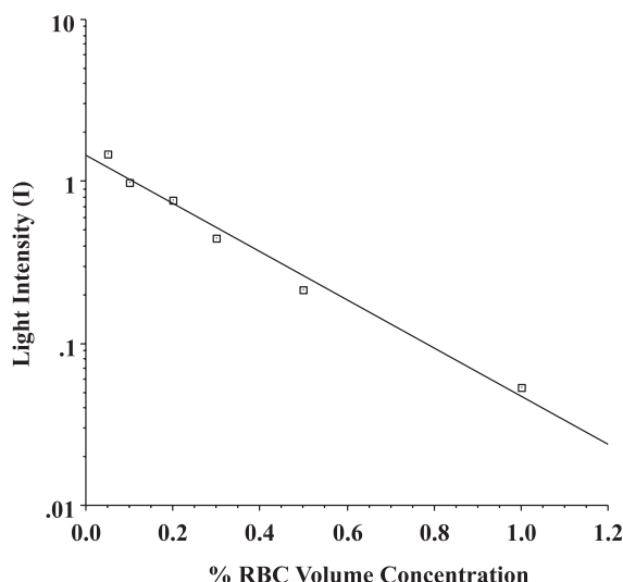
Fig. 3. The light intensity measured in the sample holder for a range of erythrocyte/isotonic saline concentrations from 0.05% to 1.0%. The slope of the line of best fit for each of the holders was similar with an overall mean of -1.653 \pm 0.172 .
